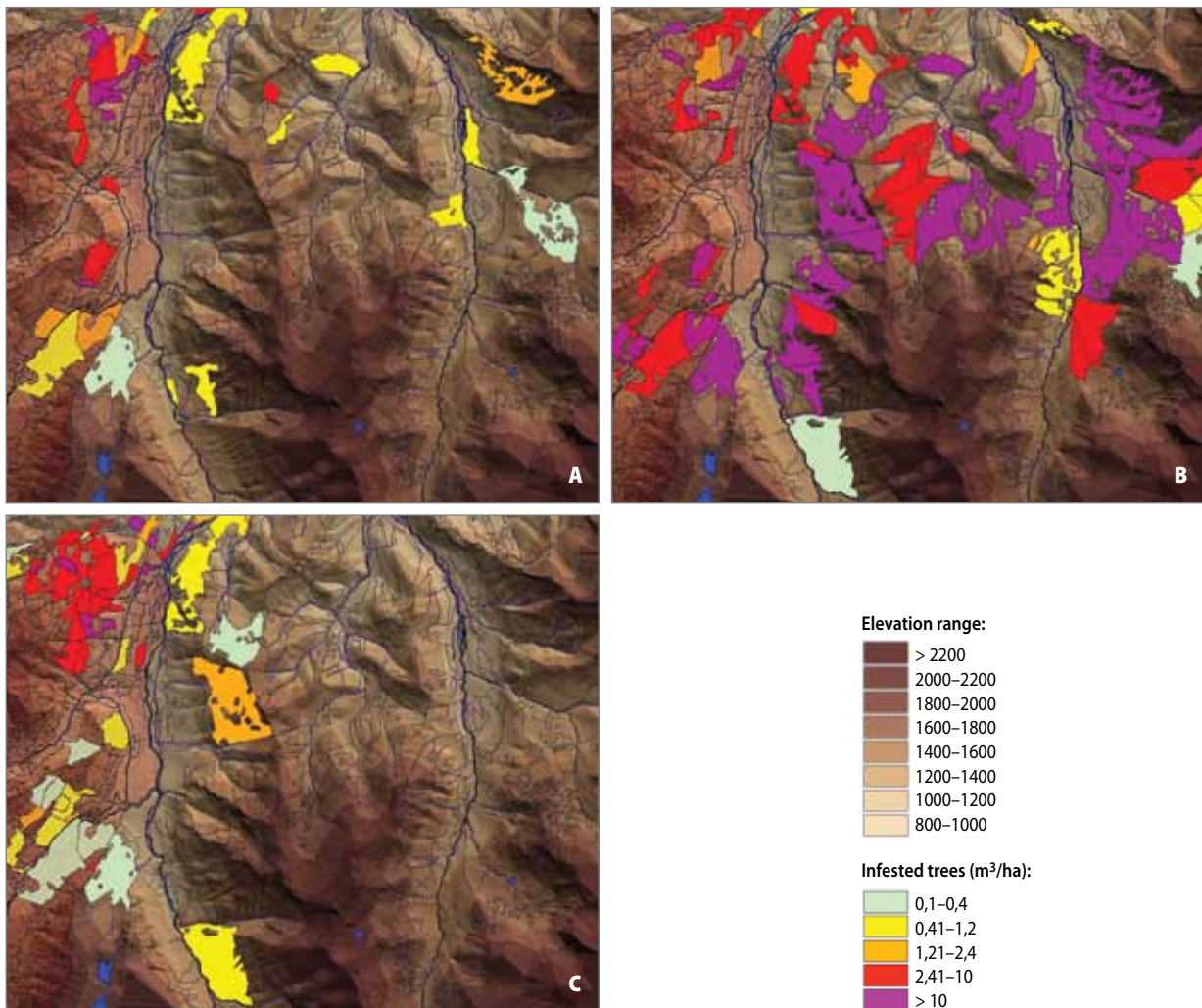
Fig. 4. Spatial development of bark beetle outbreak in the Tatra Mountains in 1991 (A), 1995 (B) and 1999 (C), with the degree of tree mortality (m 3 /ha) in individual forest sub-compartments. Passive protection zone in TPN (Poland) marked with red lines
