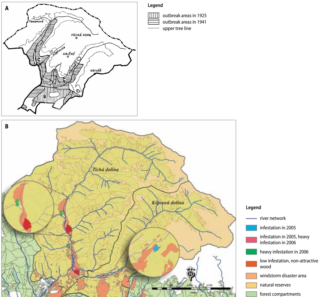
Fig. 10. Historical data on bark beetle outbreak areas in the Tichá and Koprová valley (TANAP, Slovakia) according to historical records (Zúbrik et al 2006) (A) and the results of intensive survey of bark beetles populations conducted in the autumn 2005 and 2006 (B)
