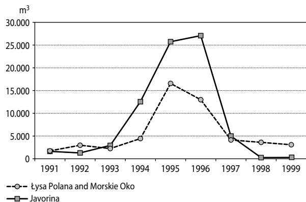
Fig. 2. Volume of trees killed by bark beetles in Polish (TPN – Lysa Polana and Morskie Oko) and Slovak (TANAP – Javorina) part of the outbreak area in the eastern Tatra Mts. in 1991–1999 (cf. Grodzki et al., 2002)
