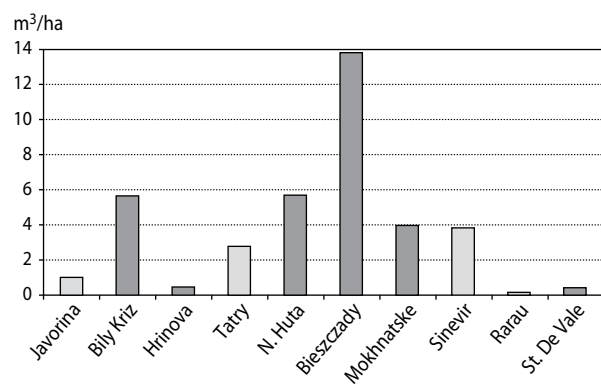
Fig. 1. The volume of infested trees ( \text{m}^3/\text{ha} ) on sites with low (grey bars) and high (dark bars) ozone concentration in 10 localities in the Carpathians (Javorina, Bílý Kříž – Czech Republic; Tatry, Bieszczady – Poland; Rarau, St. De Vale – Romania; Hriňová, Novoveská Huta – Slovakia; Mokhnatske, Sinevir – Ukraine)
